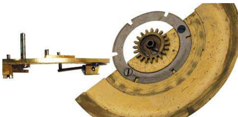
Picture 13: System for blocking the rotating mass
